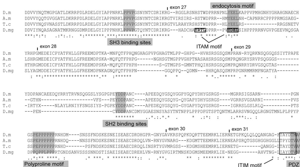
FIG. 3.—Amino acid sequence alignment of cytoplasmic tail segments of Drosophila melanogaster (D.m), Apis mellifera (A.p), Tribolium castaneum (T.c), and Daphnia magna (D.mg). Symbols represent levels of amino acid identity between species: (*) full identity, (:) strongly similar, (.) weakly similar, and ( ) no similarity. Gray squares highlight homologous regions to motifs involved in signaling pathways: SH3- and SH2-binding motifs, a polyproline motif, an endocytosis, and a PDZ motif. Black squares highlight ITIM and ITAM. The PDZ motif presents in the alternative end of the cytoplasmic tail is shown in figure 2. Exon numbers correspond to Daphnia .
