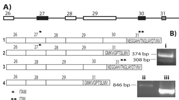
FIG. 2.—Schematic representation of Daphnia Dscam cytoplasmic tails (A) Daphnia magna tail structure and splicing possibilities result in 4 alternative forms. Exons 26–31 code for the cytoplasmic tail. Exons 27 and 30 can be included in the mRNA or skipped. C-terminal end of the cytoplasmic tail changes if exon 30 is included (1) or skipped (3). Two other forms, (2) and (4), are obtained through the inclusion or exclusion of exon 27. (B) Daphnia magna Dscam cytoplasmic tail expression in the whole-body mRNA. (i) The 2 bands correspond to the cDNA fragments that can be coded by exons 29–31. The bigger fragment includes exons 29, 30, and 31 and the smaller includes exons 29 and 31. (ii) Fragment corresponds to cDNA containing exons 27–31. Cloning and sequencing of this fragment revealed that exon 30 may or may not be transcribed. (iii) Control: whole-body mRNA actin expression.
