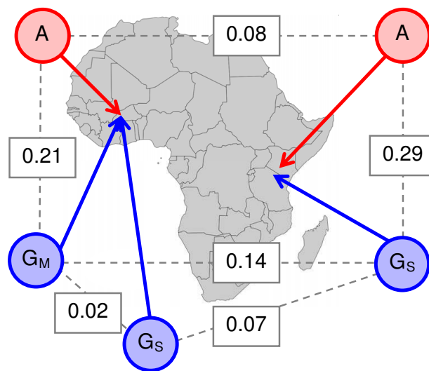
Figure 2 Genetic differentiation between populations. Arrows indicate approximate sampling locations within Africa, and letters identify species (A- An. arabiensis , G- An. gambiae , M-form and S-form). Dashed lines indicate pairs of populations for which genetic differentiation was calculated, and numbers are K_{ST} statistics, averaged across all 32 loci.
