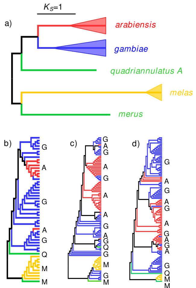
Figure 3 Genetic divergence within the gambiae species complex. (a) An un-rooted neighbour-joining tree, calculated from pairwise K_S between species averaged across loci. Branch lengths are to scale. The filled triangles illustrate the relative scale of diversity and divergence within the complex, such that the length of the triangle is half the divergence between haplotypes within species (i.e. \pi_s/2 ) and net divergence ( K_S - \pi_s ) corresponds to branch-lengths that are not part of the triangle. (Note that population samples and thus \pi_s were not available for An. quadriannulatus A and An. merus ). (b)-(d) Neighbour-joining cladograms (i.e. topology only, branch-lengths uninformative) showing the unique alleles sequenced from three loci. Note that in all cases An. gambiae and An. arabiensis alleles are intermixed. (b) to (d) are control locus 14, SRPN7 and SRPN11, selected to illustrate a wide range of K_{ST} values between An. gambiae and An. arabiensis ( K_{ST} = 0.51, 0.10 and 0.09 , respectively).
