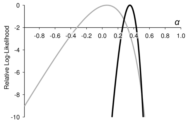
Figure 4 The power to estimate \alpha using An. gambiae and An. arabiensis . The relative log-likelihood of \alpha (the proportion of amino-acid substitutions that are adaptive) estimated using the modified McDonald-Kreitman approach [30]. The grey curve is calculated from all 102 genes for which both An. arabiensis and An. gambiae population samples were available in the dataset of Cohuet et al. [6]. The black curve shows an equivalent dataset of 102 genes from Drosophila melanogaster and D. simulans , with genes selected to be the same average length as those in the Cohuet dataset (D. J. Obbard, J. J. Welch and F. M. Jiggins, unpublished data). Despite both pairs of species having similar levels of diversity ( \pi_S from 1.6% to 2.9%), for the Anopheles dataset the bounds (2 units of log Likelihood) stretch from -0.33 to 0.32 (and include zero) while for Drosophila the bounds only stretch from 0.26 to 0.44, and the maximum-likelihood estimate of \alpha is 35%. The low precision in the second estimate reflects the very low power available due to the low divergence in An. gambiae - An. arabiensis comparisons
